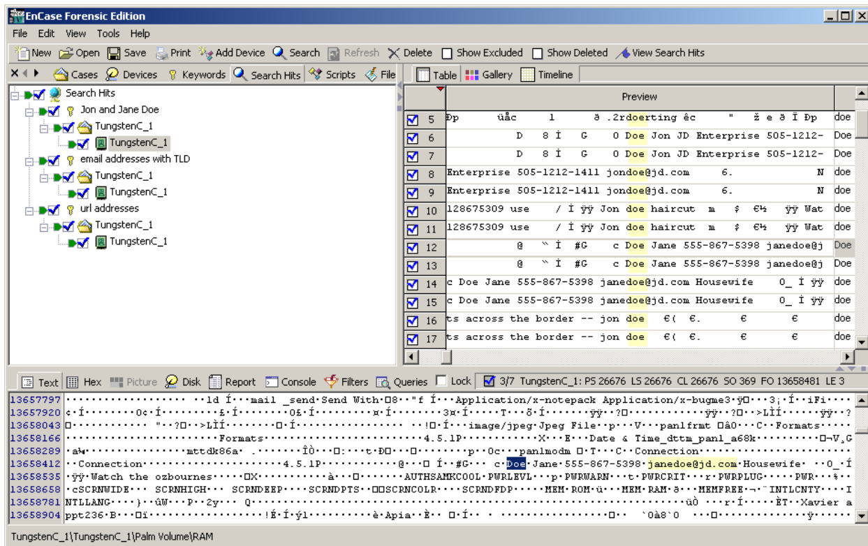
Figure 18: Search Results
