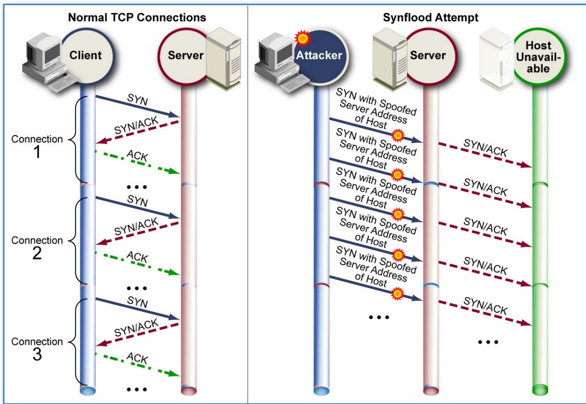
Figure 4-4. Synflood Attack
