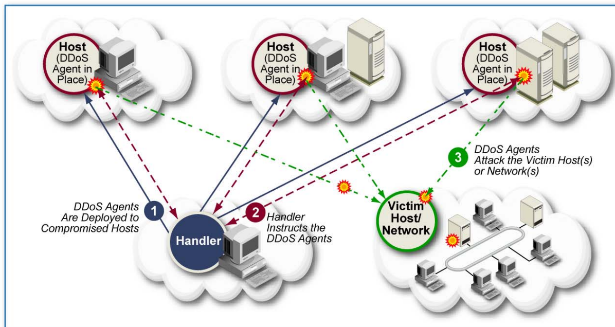
Figure 4-3. Distributed Denial of Service Attack
