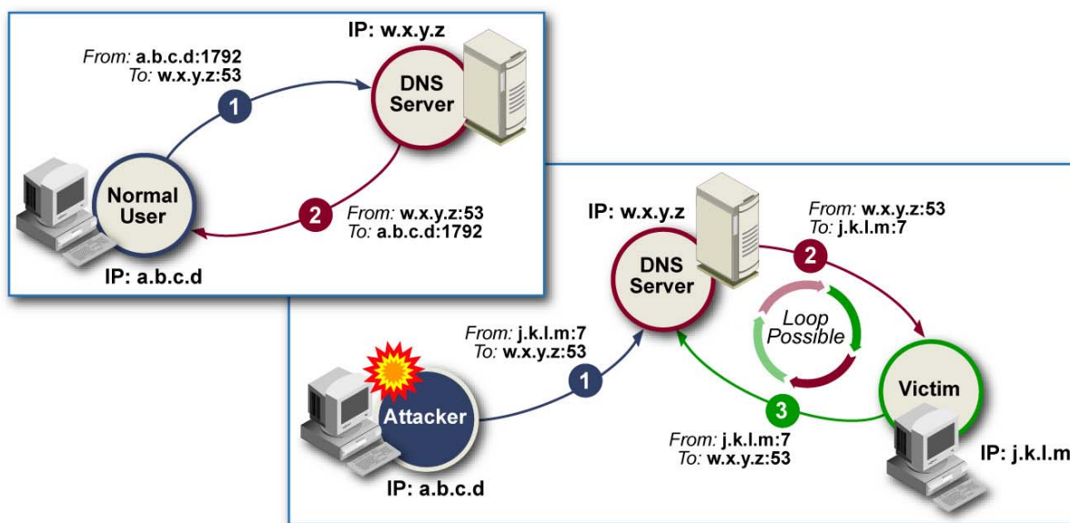
Figure 4-1. Reflector Attack Using a DNS Server
