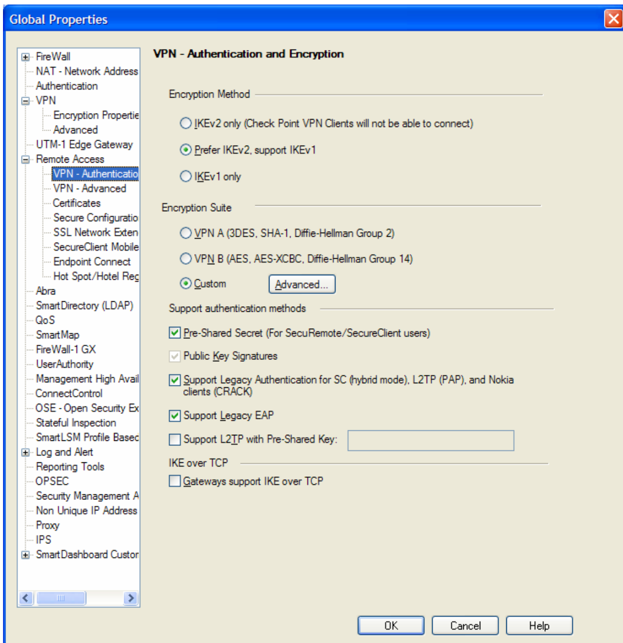
Figure 5 – Only Pre-Shared Keys or Digital Certificates may be used to Authenticate Clients
