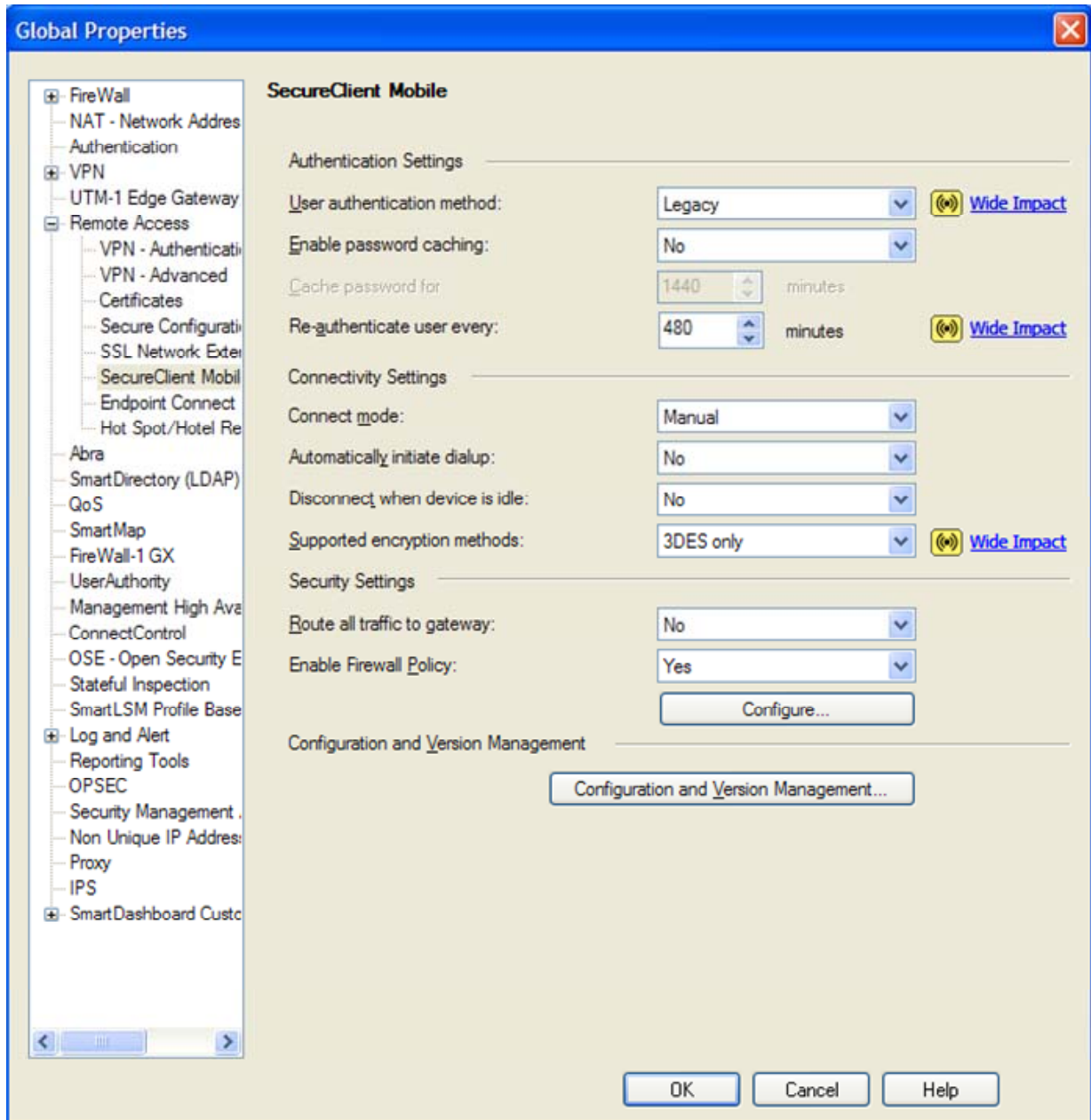
Figure 9 – Only FIPS-Approved Algorithms may be used with TLS
