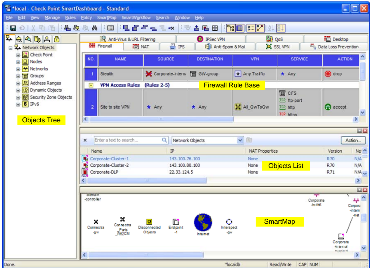
Figure 2. – Easy to Use Management Tools
