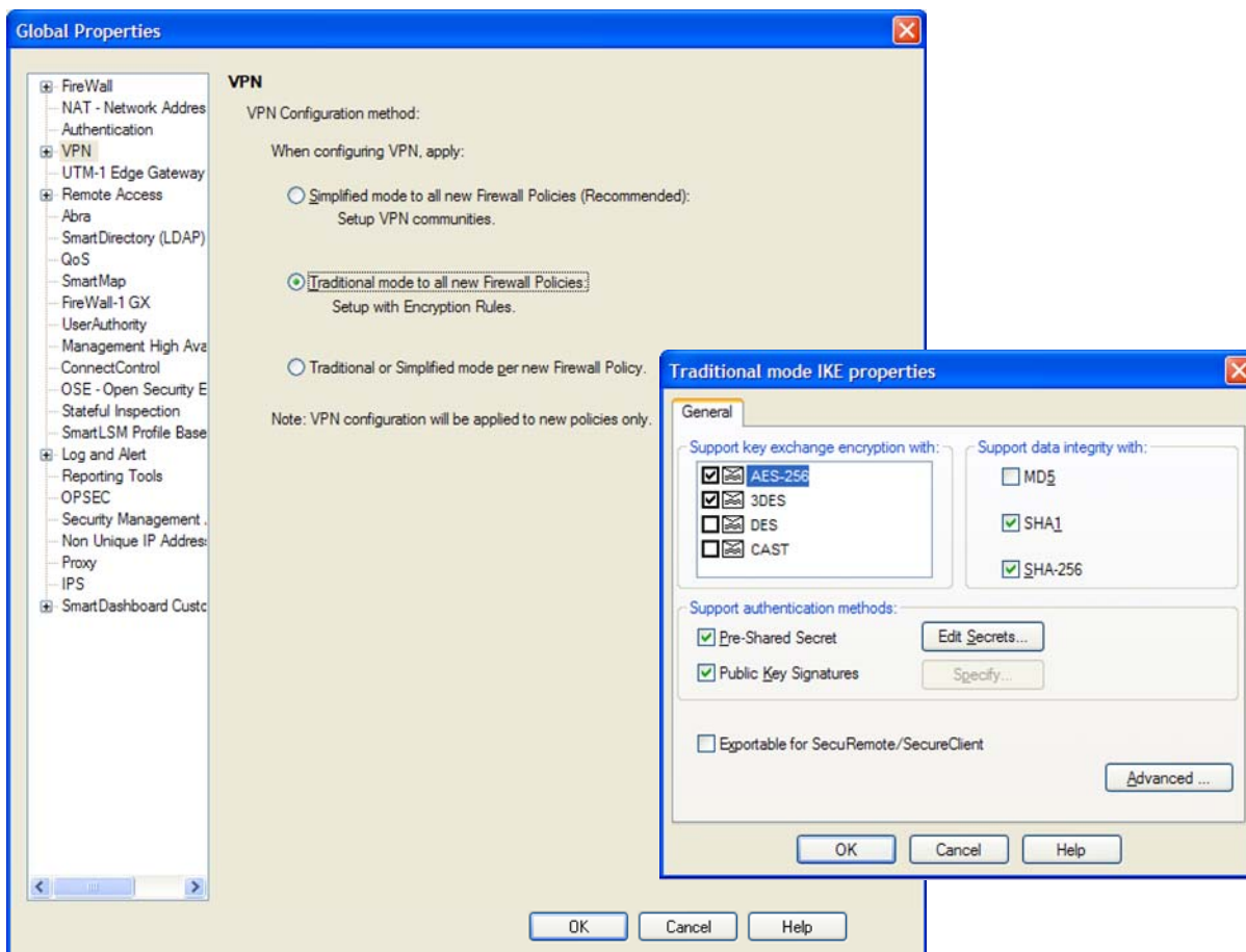
Figure 3 – In Traditional Mode, Select Only FIPS-Approved Algorithms for use with IKE
