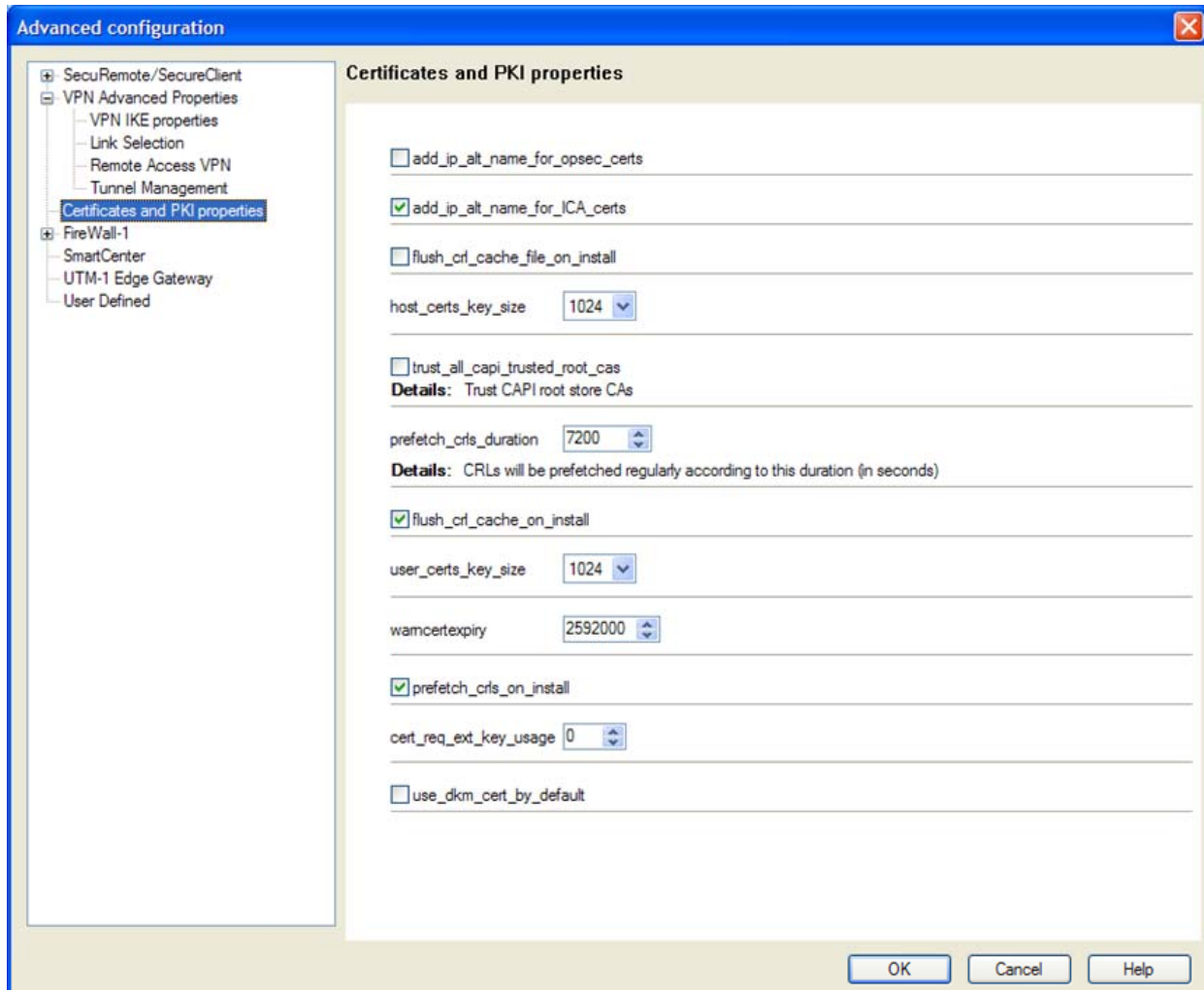
Figure 10 – Configuring the module to enable Distributed Key Management (DKM) globally
