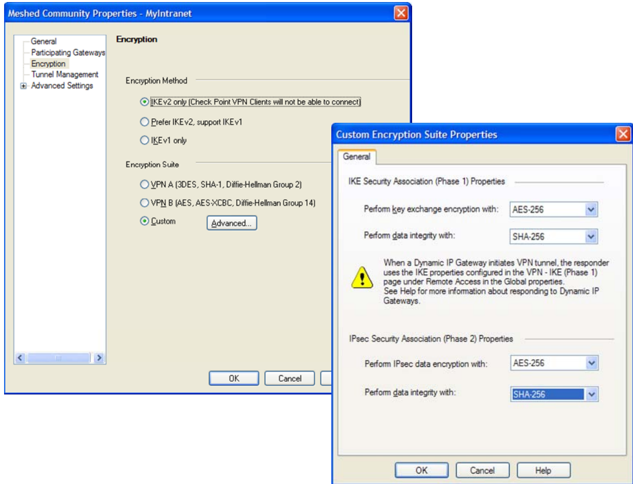
Figure 4 – In Meshed Communities Select Only FIPS-Approved Algorithms for use with IKE
