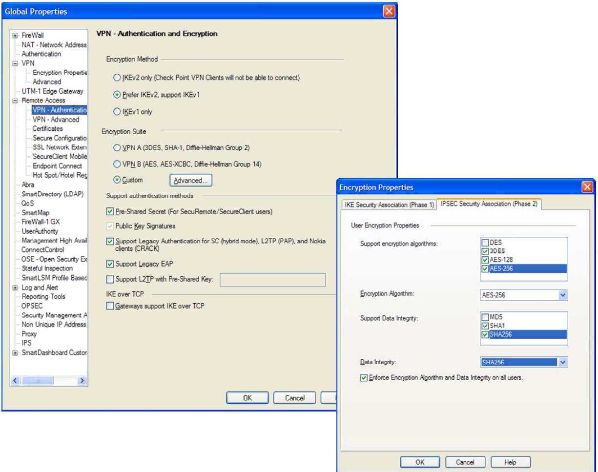
Figure 7 – Only FIPS-Approved Algorithms may be used with IPsec
