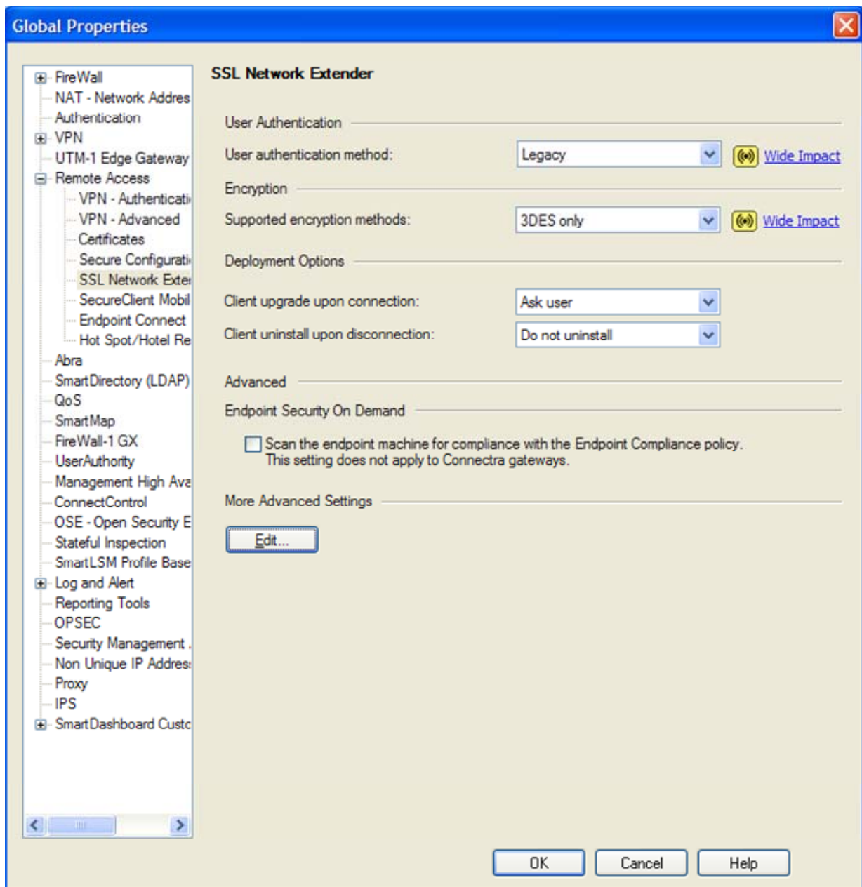
Figure 8 – Only FIPS-Approved Algorithms may be used with TLS
