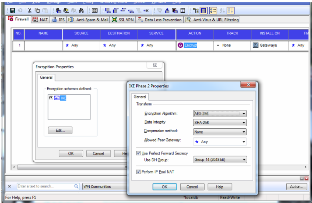
Figure 6 – Only FIPS-Approved Algorithms may be used with IKE (Phase 2)
