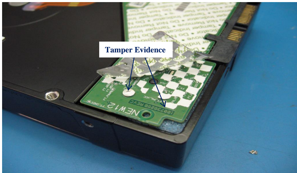
Figure 9: Enterprise Capacity® 3.5, HDD v4 (SAS/SATA) PCBA Tamper Evidence
