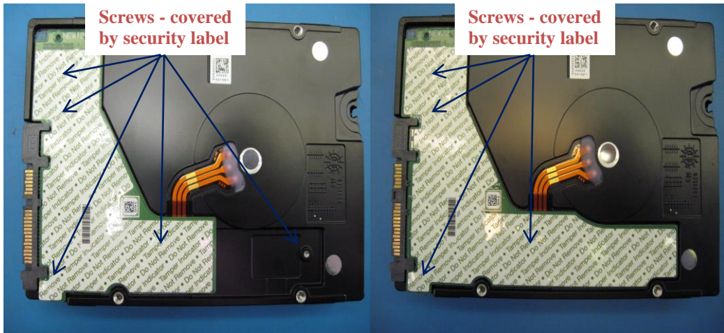
Figure 10: Enterprise Capacity® 3.5, HDD v4 (SAS/SATA) Screw covered by Security label
