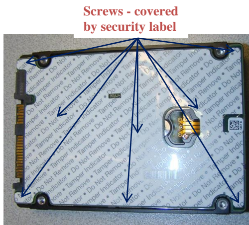
Figure 12: Enterprise Performance® 2.5, HDD v8(SAS) Screw covered by Security Label
