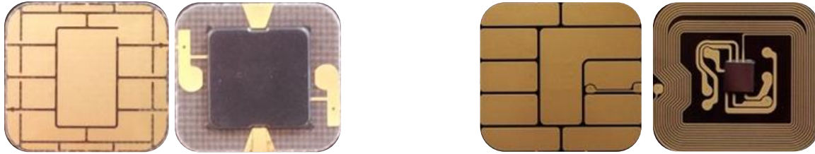
Figure 2 – Dual interface: P-M8.4-8-3 front and back (left); S-COM6.8 front and back (right)
