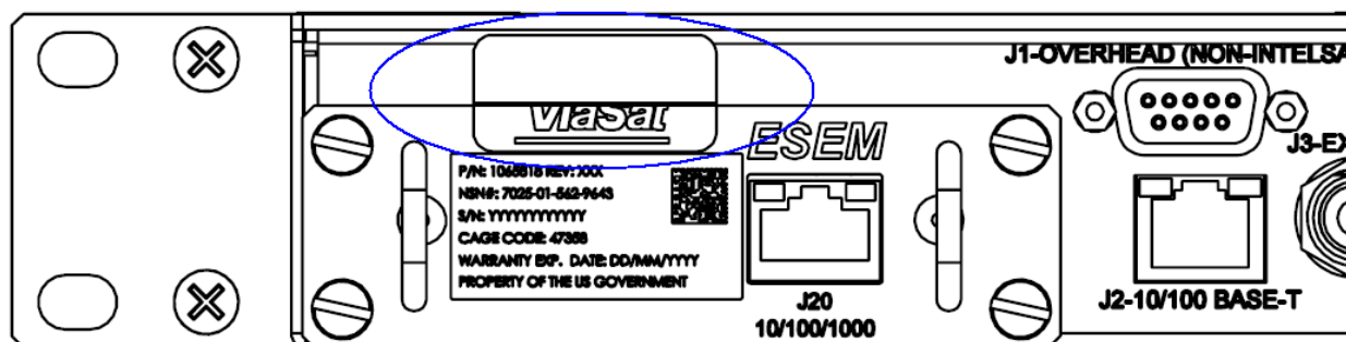
Figure 6: Tamper Seal Location on Expansion Port with ESEM Installed (1 Seal)
