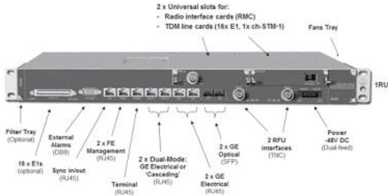
Figure 10 - PTP 820GX Interfaces
