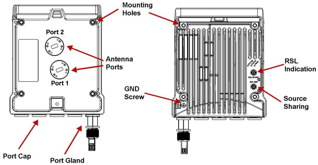
Figure 11 - PTP 820C Interfaces (Front and Back)
