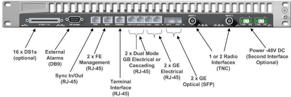
Figure 9 - PTP 820G Interfaces
