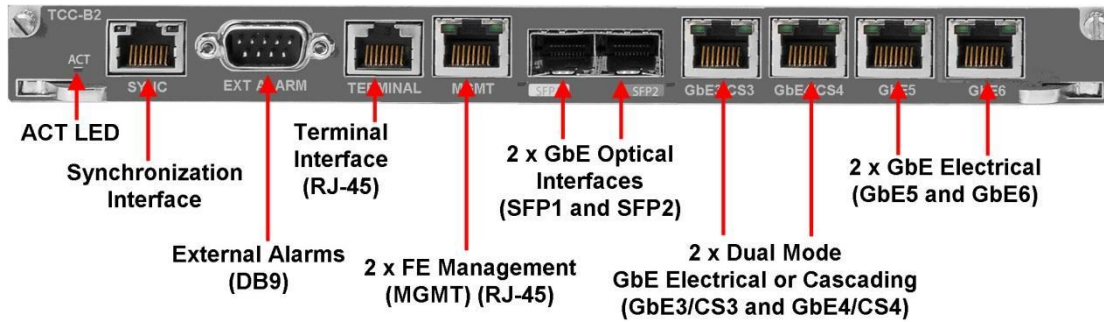
Figure 7 - PTP820 TCC-B2: N000082H002 and PTP820 TCC-B2-XG-MC: N000082H003 Interfaces
