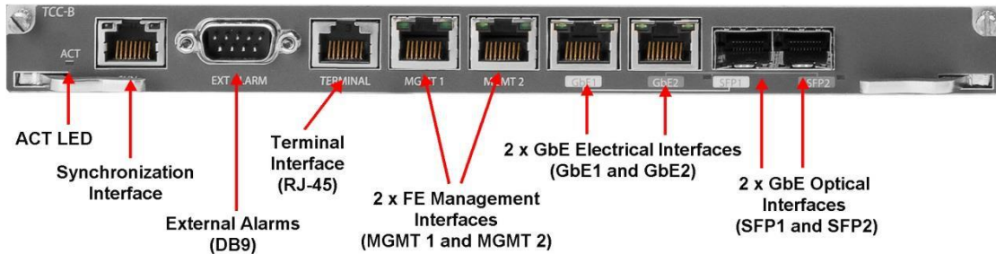
Figure 6 - PTP820 TCC-B-MC: N000082H001 Interfaces
