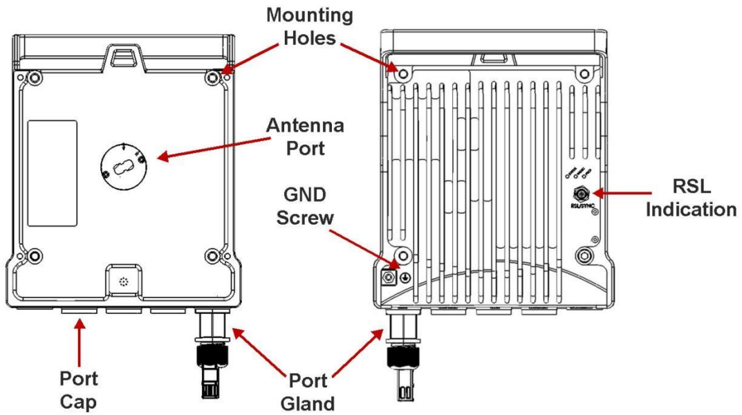
Figure 12 - PTP 820S Interfaces (Front and Back)
