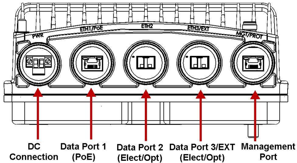
Figure 13 - PTP 820C and PTP 820S Interfaces Side
