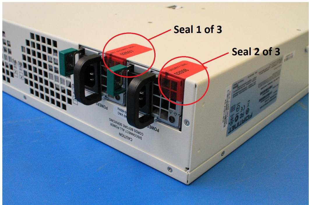
Figure 6: FortiGate-1500D Enclosure Seal, top, left side
