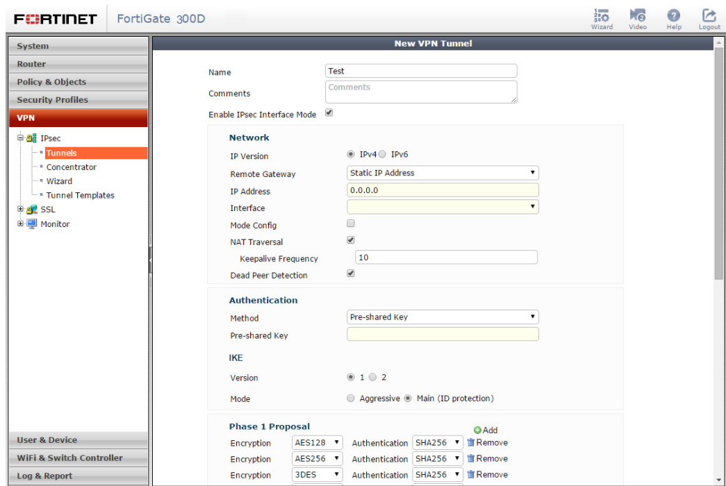
Figure 3: The FortiGate web-based manager
