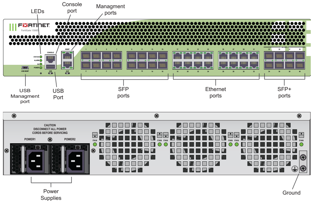
Figure 2: FortiGate-1500D Front and Rear Panels
