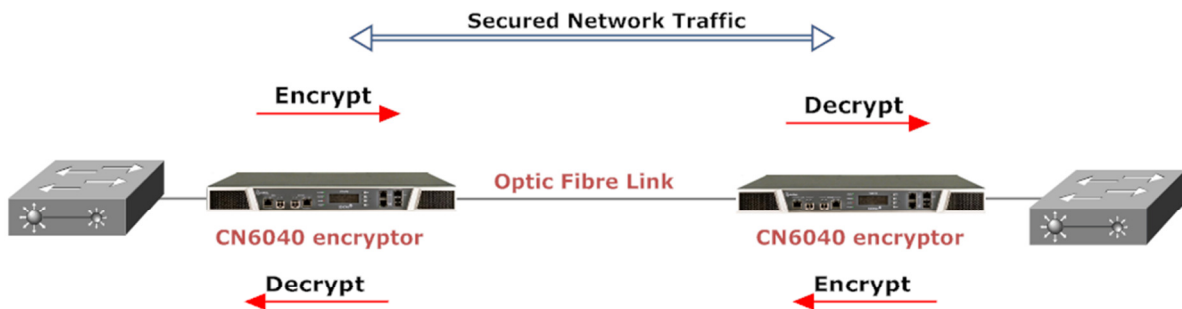
Figure 2 – CN6040 Operational Overview
