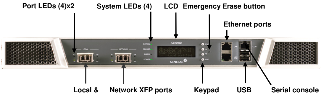
Figure 12 - Front View of the CN6100 [O] Encryptor
