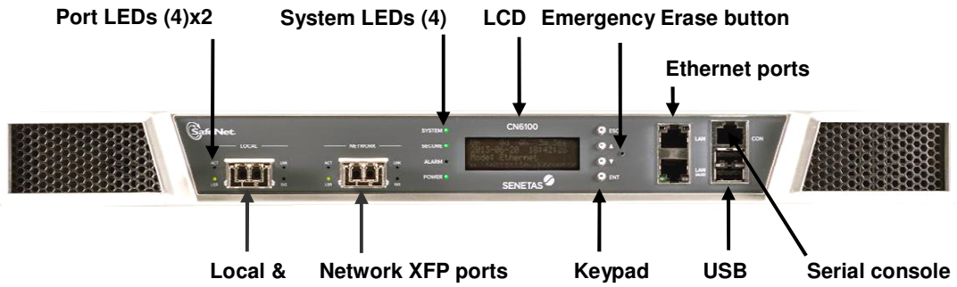
Figure 11 - Front View of the CN6100 [Y] Encryptor
