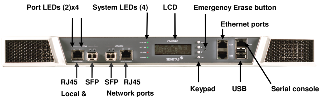
Figure 10 - Front View of the CN6040 [O] Encryptor
