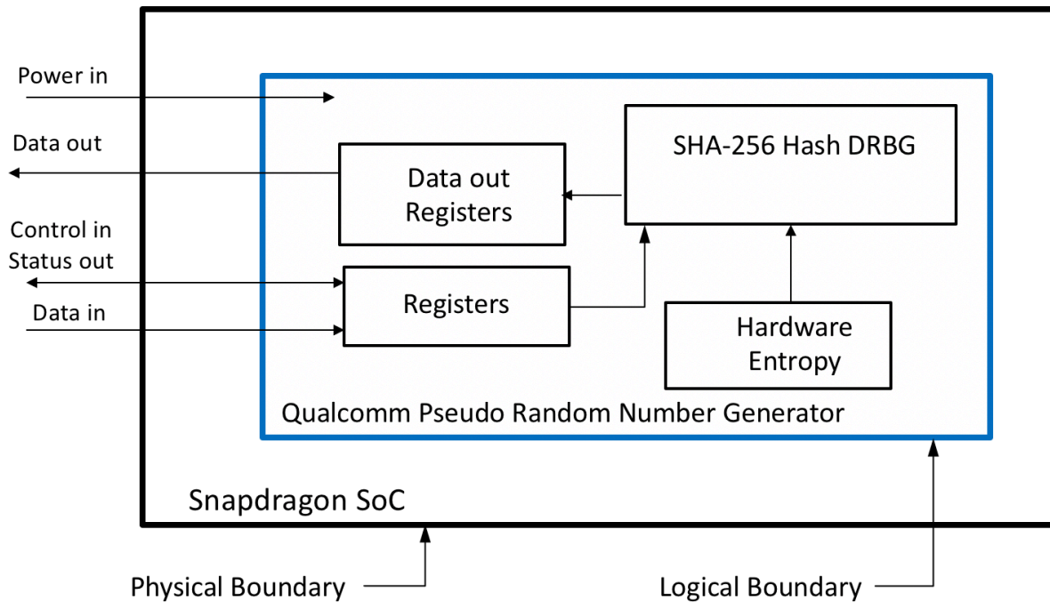
Figure 1: Cryptographic Boundary
