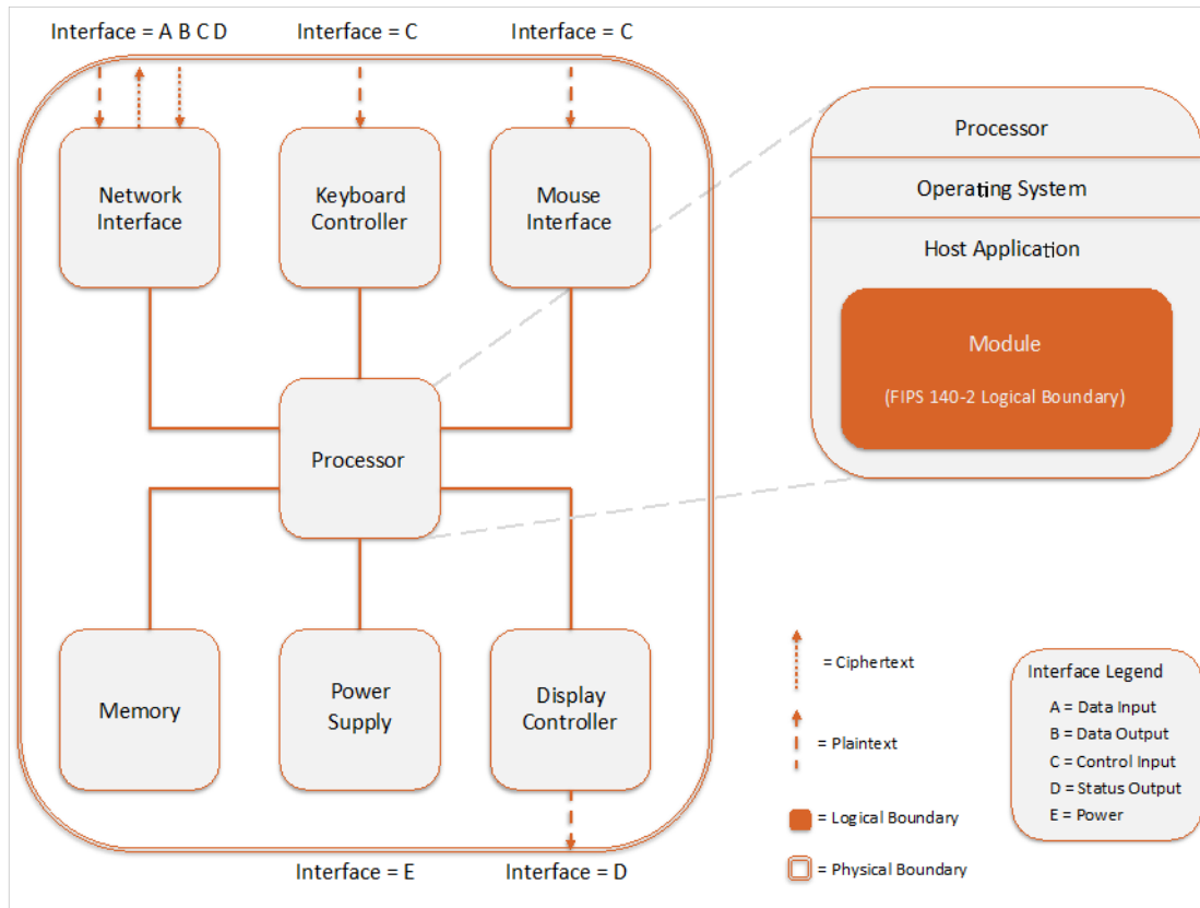
Figure 1 – Module Boundary and Interfaces Diagram
