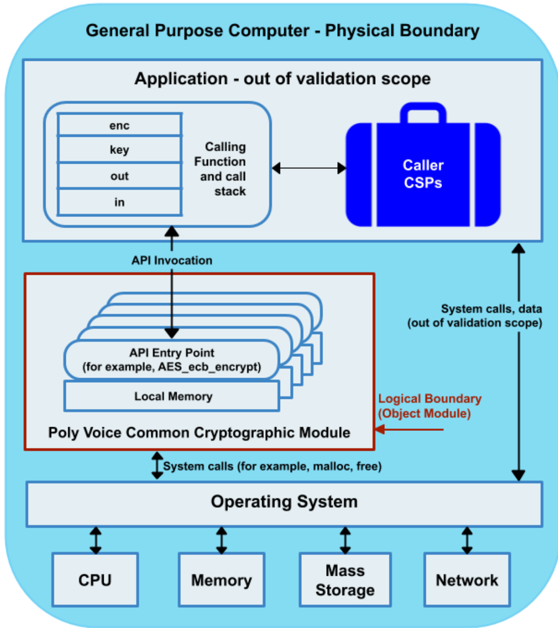
Figure 1 - Module Block Diagram
