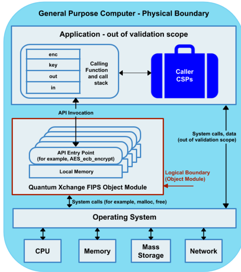
Figure 1 - Module Block Diagram
