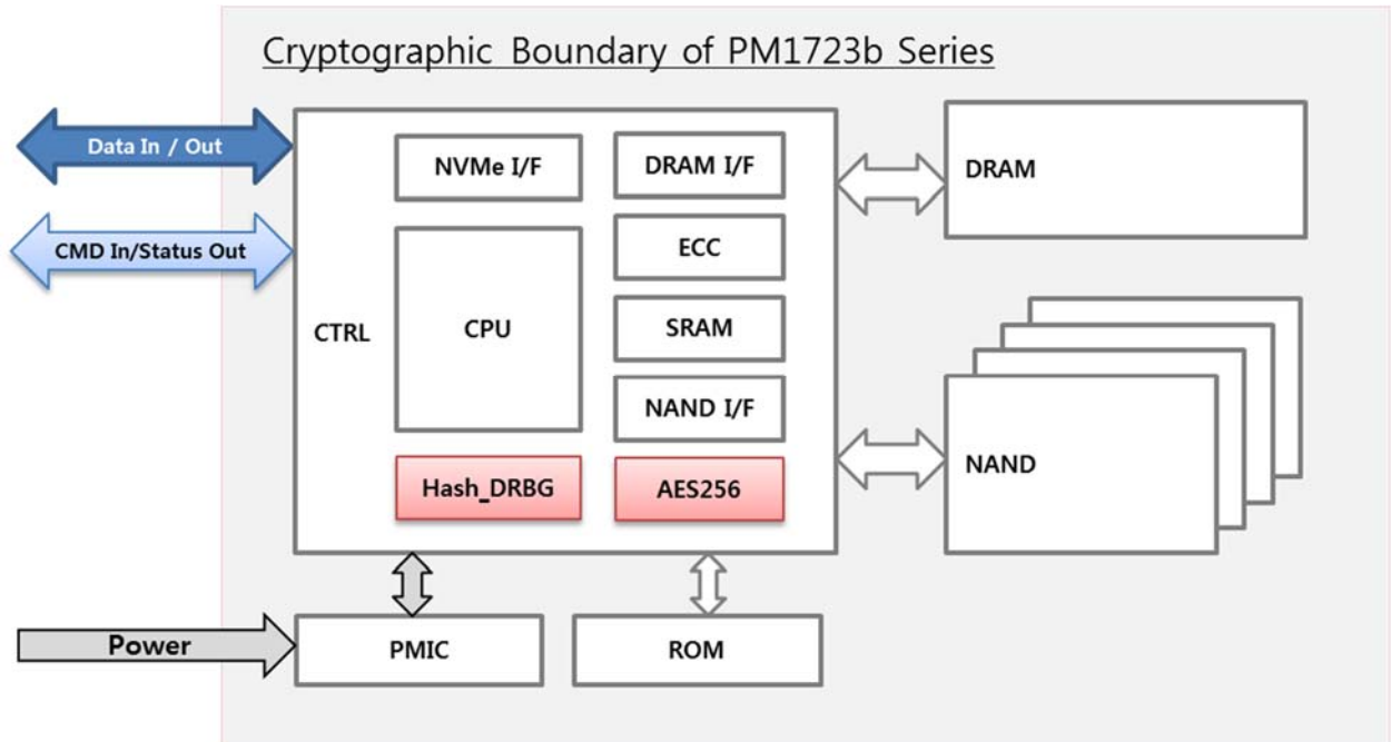
Exhibit 5 – Block Diagram for Samsung NVMe TCG Opal SSC SEDs PM1723b Series.
