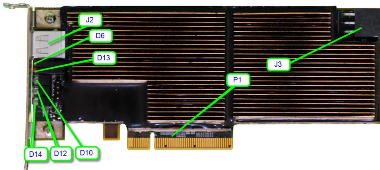
Figure 1 – Top View of the Cryptographic Module
