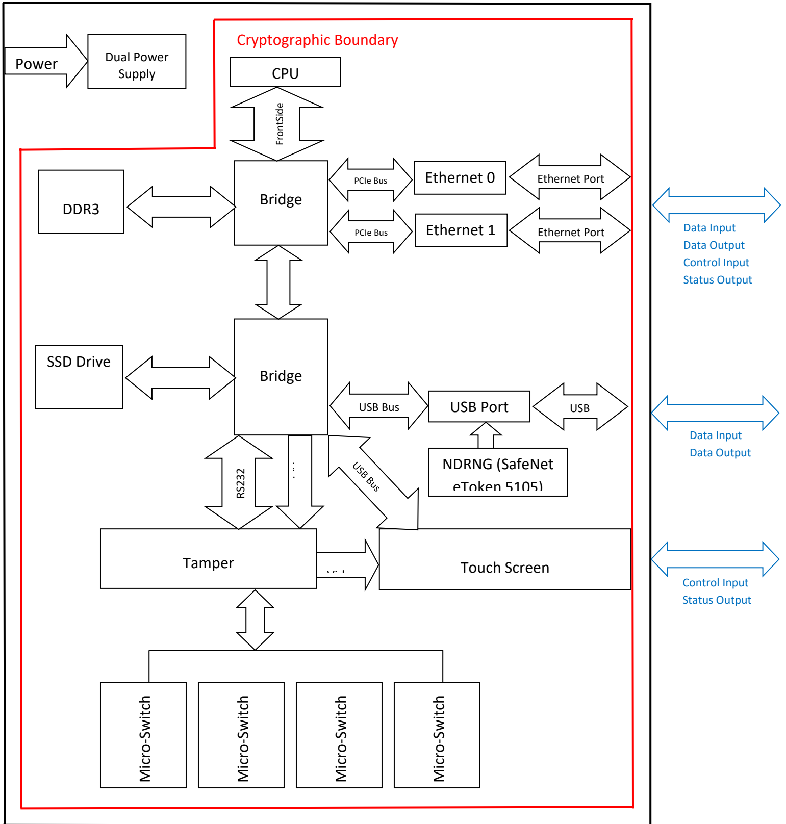
Figure 3 - DSA Hardware Block Diagram
