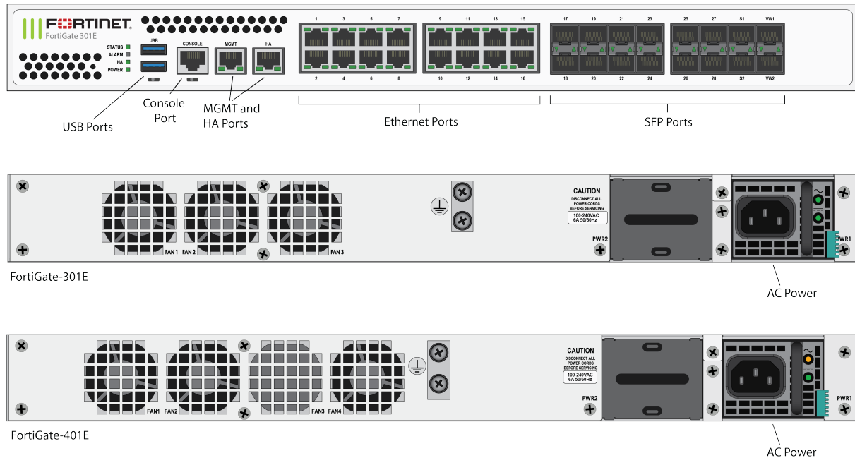
Figure 2 - FortiGate-301E and 401E Front and Rear Panels
