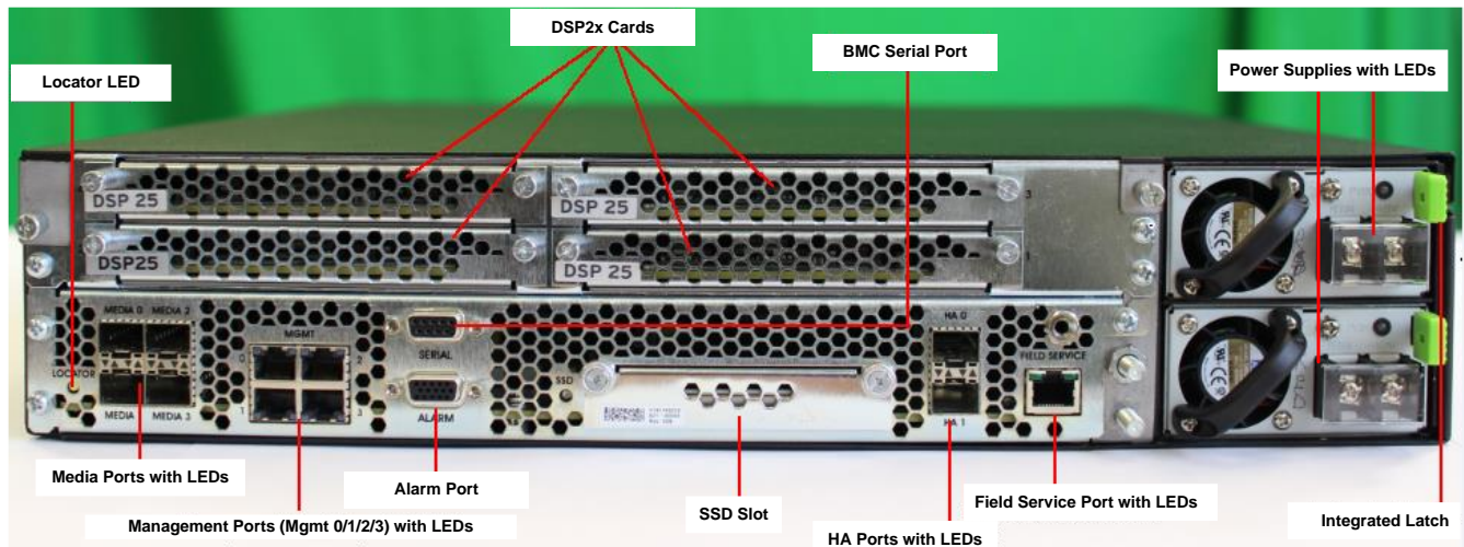
Figure 5 – Rear Panel Ports/Interfaces and LEDs
