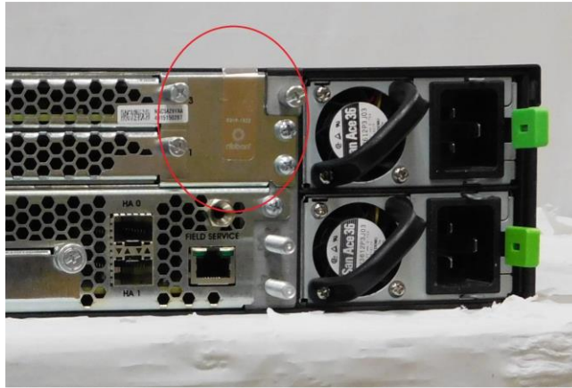
Figure 8 – Label 3 Placement (Rear of Chassis)
