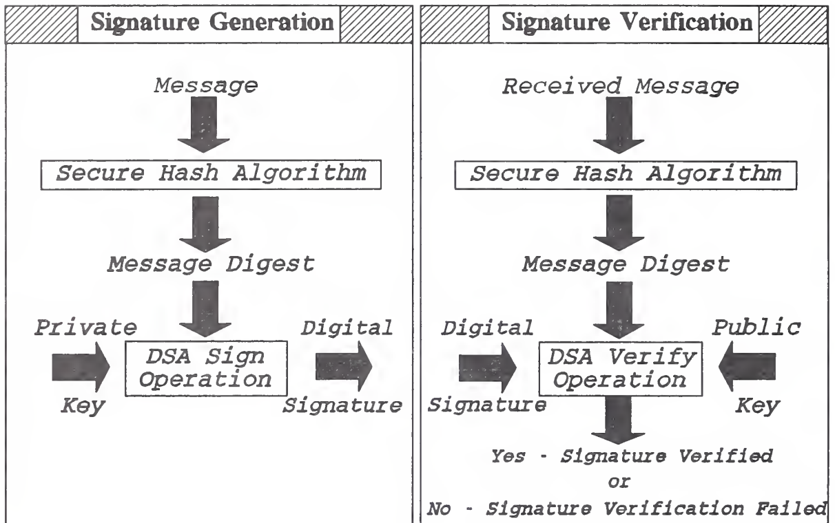
Figure 1: Using the SHA with the DSA
