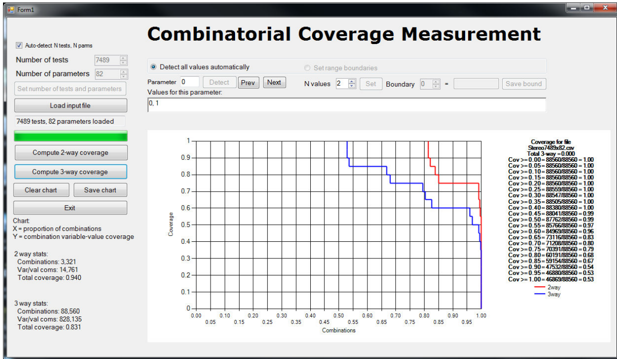
Figure 4. Coverage Measurement Tool user interface.
