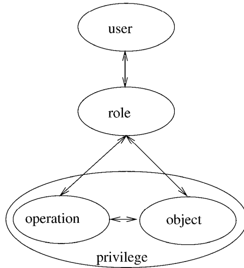
Fig. 1. Role-Operation-Object Relationship
