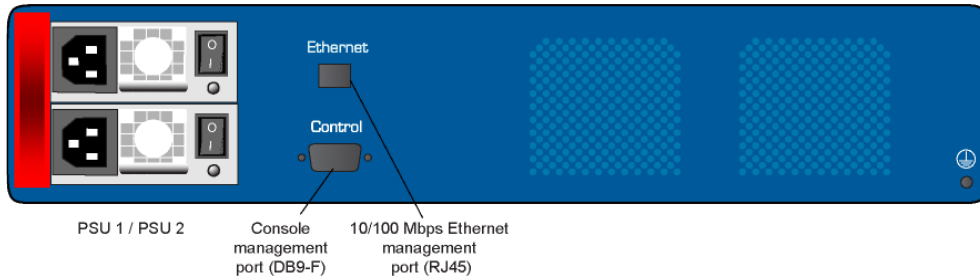
Figure 4-9 1600x437, Rev. 01 Top
