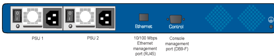
Figure 4-5 1600X433, Rev. 02 Rear
