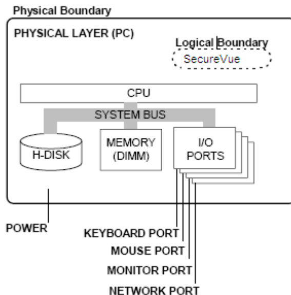
Figure 1 - Cryptographic Boundary
