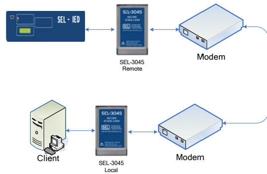
Figure 2: Point to Point Network
