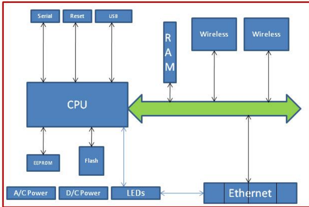
Figure 2 – IntelliCom WAN® 1720 Wireless Mesh Nodes Block Diagram
