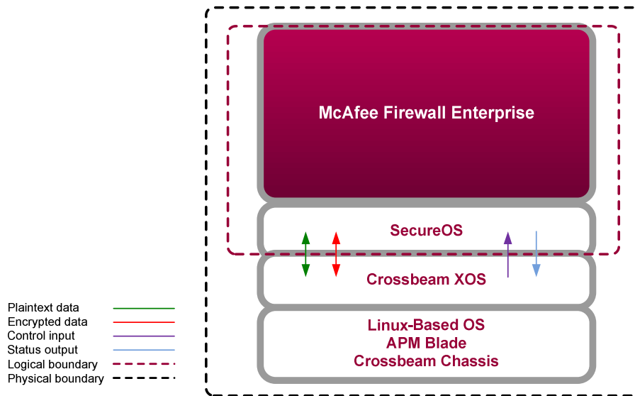
Figure 3 – MFE Virtual Appliance Cryptographic Boundaries
