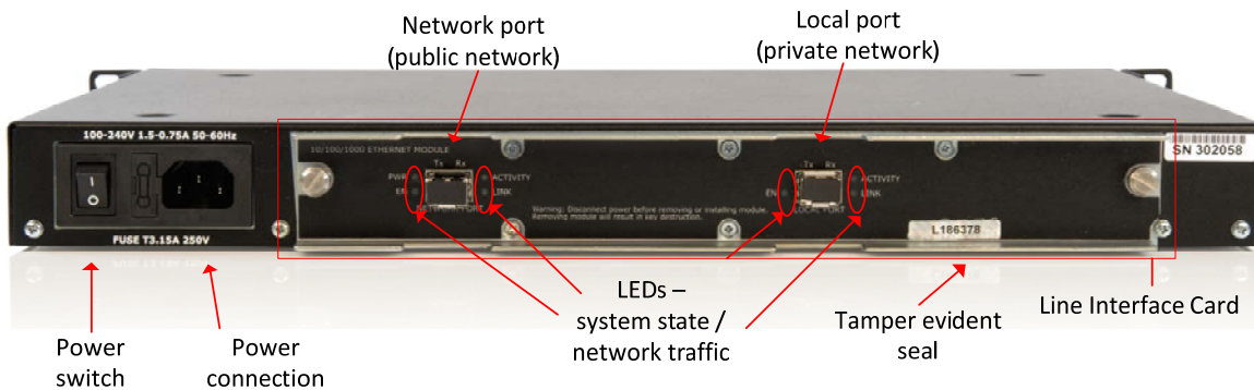
Figure 2.2-2 – Rear View of Model 600 SafeNet Encryptor
