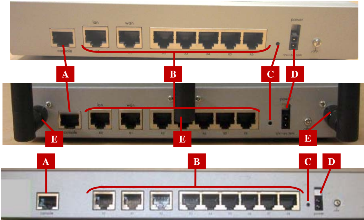
Figure 2 – NSA 220 (Top), 220W (Middle) and 240 (Bottom) Back Panels
