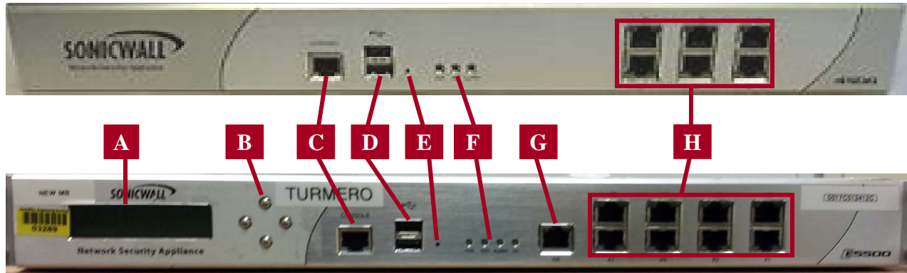
Figure 1 – NSA 4500 (Top) and E5500 (Bottom) Front Panels
