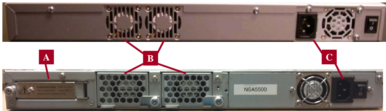
Figure 2 – NSA 4500 (Top) and E5500 (Bottom) Back Panels
