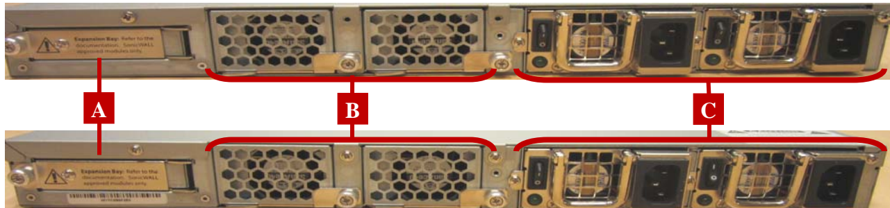
Figure 2 – NSA 8500 (Top) and NSA 8510 (Bottom) Back Panels
