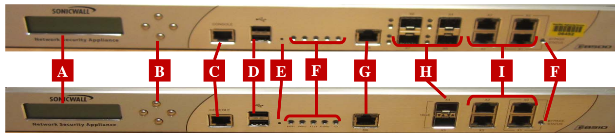
Figure 1 – NSA 8500 (Top) and NSA 8510 (Bottom) Front Panels
