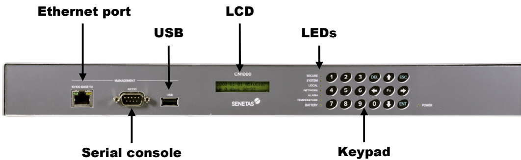
Figure 10 - Front View of CN1000 models A5141B [O], A5165B [O], A5175B [O]
