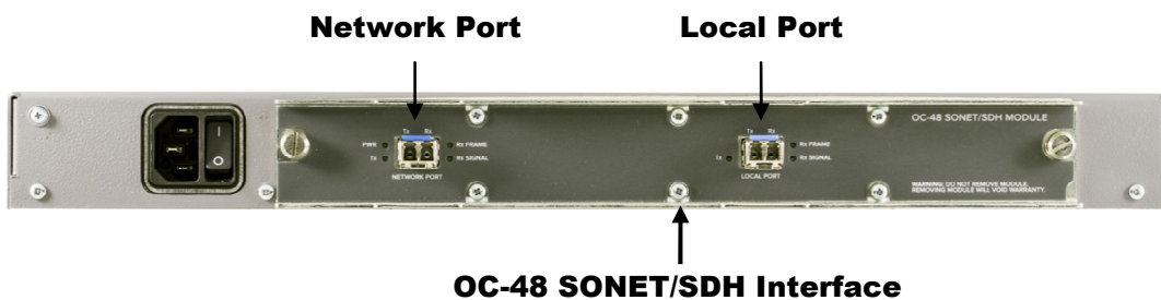
Figure 13 - Rear view OC-48/STM-16 SONET/SDH models A5165B [Y] and A5165B [O]
