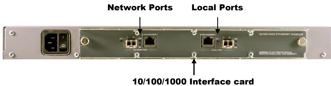
Figure 12 - Rear view 1G Ethernet models A5141B [Y] and A5141B [O]
