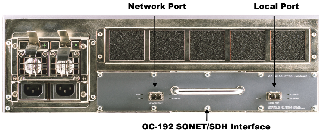
Figure 19 – Rear view of CN3000 OC-192/STM-64 – SONET/SDH Interface AC models A5213B [Y], A5213B [O]
