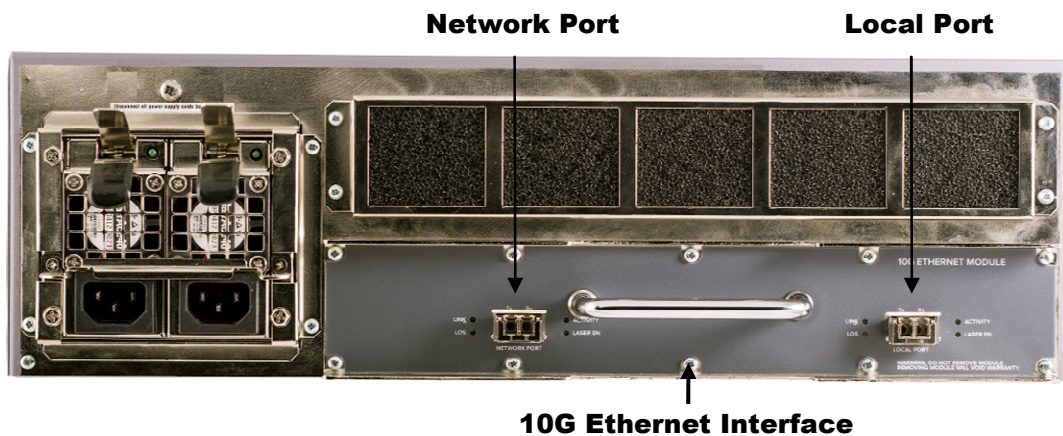
Figure 18 – Rear view of CN3000 10G Ethernet Interface AC models A5203B [Y], A5203B [O]
