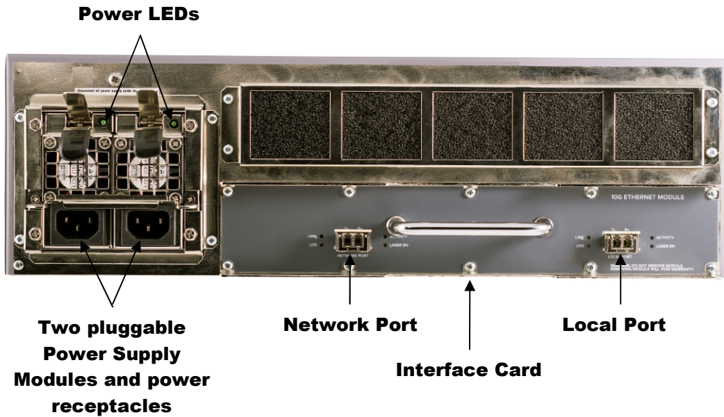
Figure 17 - Rear View of CN3000 Series
