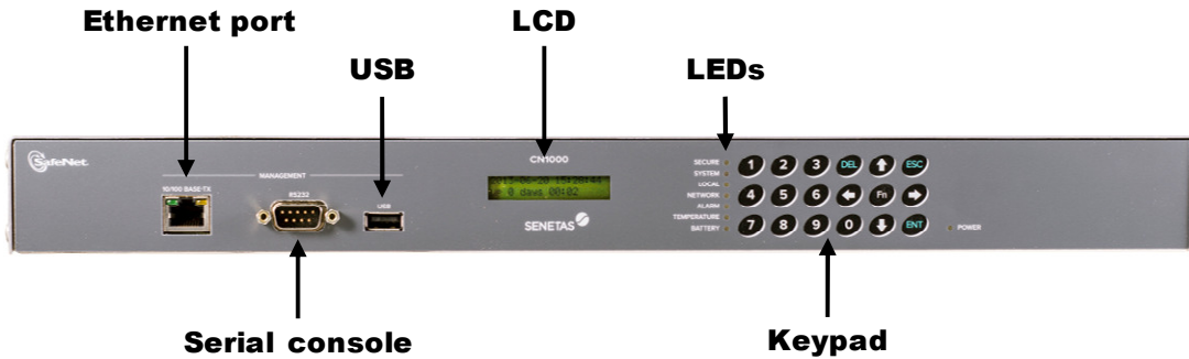
Figure 9 - Front View of CN1000 models A5141B [Y], A5165B [Y], A5175B [Y]
