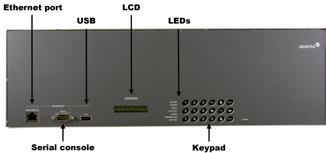
Figure 15 - Front View of CN3000 models A5203B [Y], A5204B [Y], A5213B [Y], A5214B [Y]
