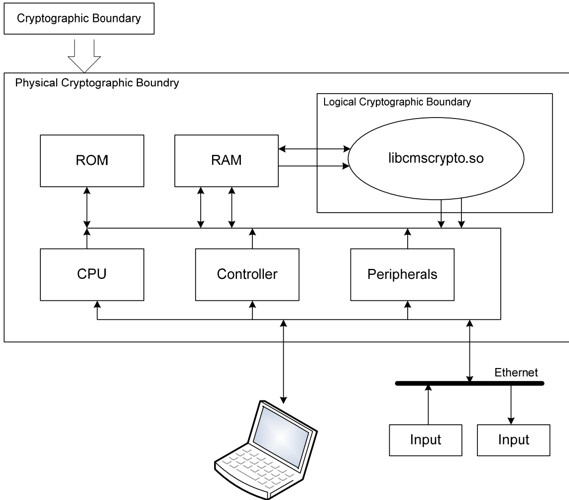
Figure 1: Block diagram of hardware and software components
