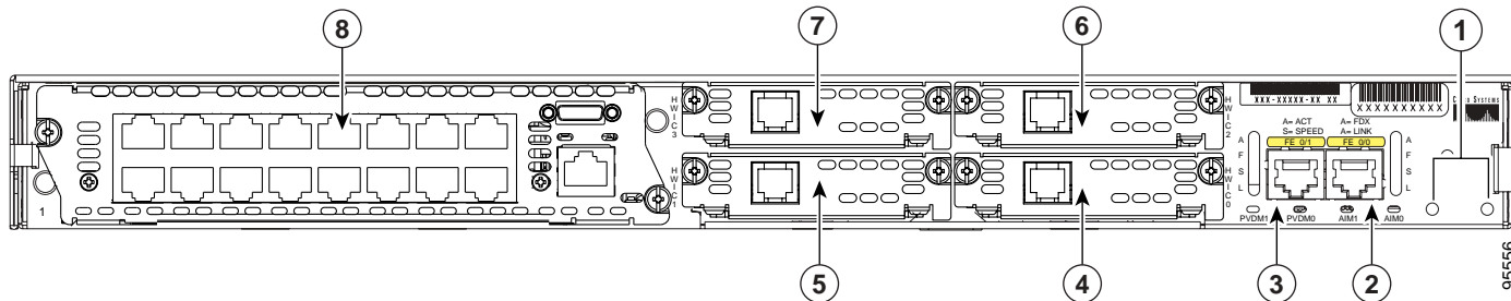
Figure 3 Cisco 2811 Rear Panel Physical Interfaces
