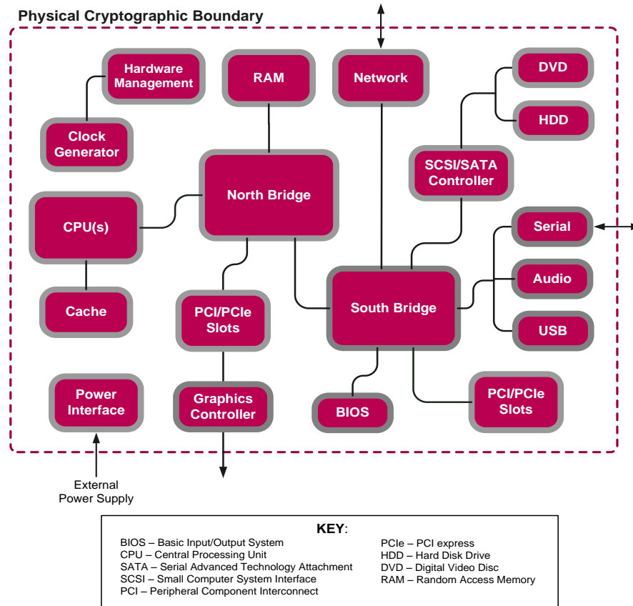
Figure 3 – Block Diagram for the WG 5000 and WG 5500
