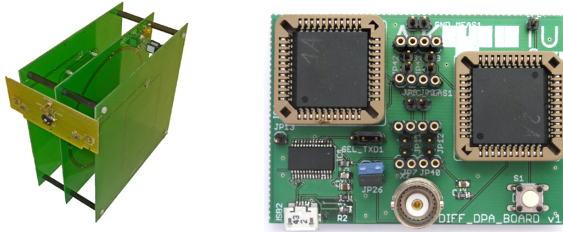
Fig. 5. The test apparatus according to the ISO/IEC 10373-6 standard [5]. Fig. 6. The AT89S8253 evaluation board.
