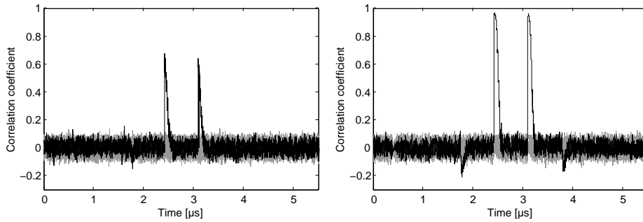
Fig. 10. Result of a classical CPA attack on one ATmega128 device (reference attack). Fig. 11. Result of a CPA attack that exploits the difference of two side channels (difference attack).
