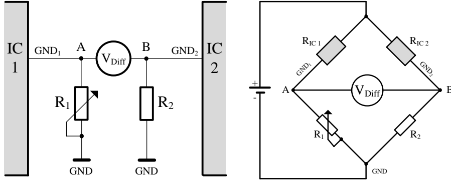
Fig. 1. Schematic of proposed apparatus. Fig. 2. Schematic of a Wheatstone bridge.
