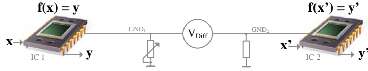
Fig. 9. The processing of different input data x and x' causes a voltage difference between both ICs which can be exploited in a side-channel attack.
