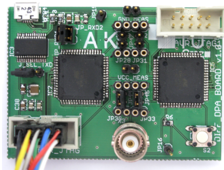
Fig. 7. The ATmega128 evaluation board.
