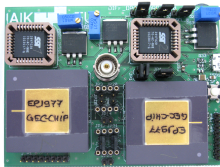
Fig. 8. The GRANDESCA-chip evaluation board.
